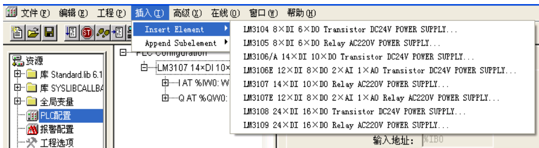
图 2-3-11 “插入”菜单 (2)
